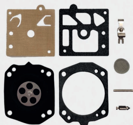
KIT REPARO DO CARBURADOR GX100/GXR120 KRWF/KRW CÓD: HM501005
